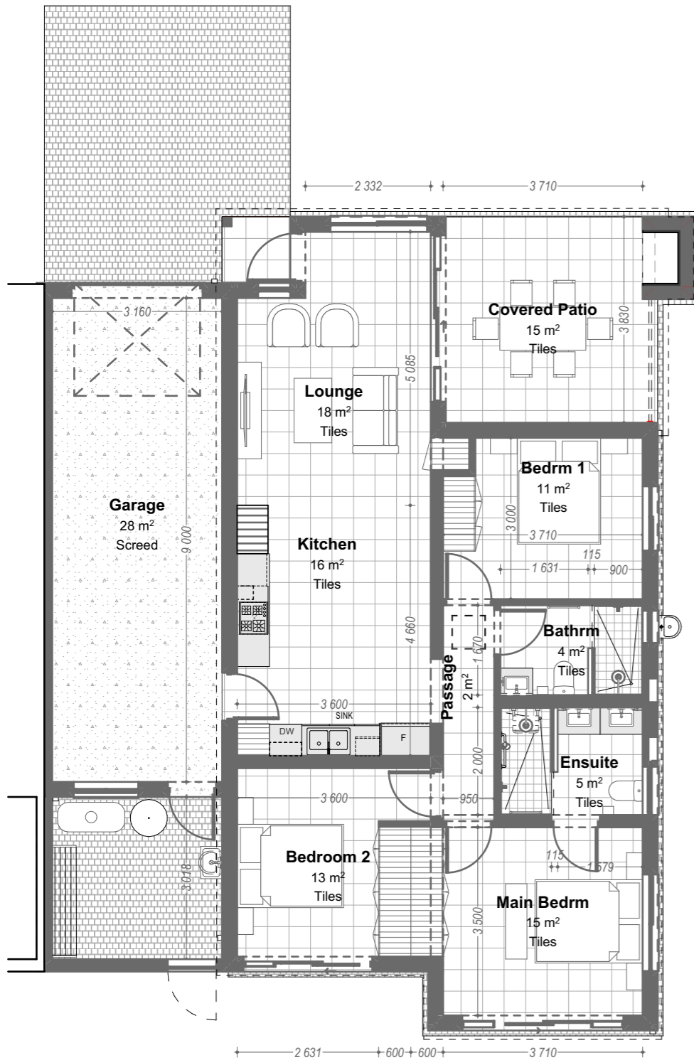
General Floor Plan - S2 1:100
