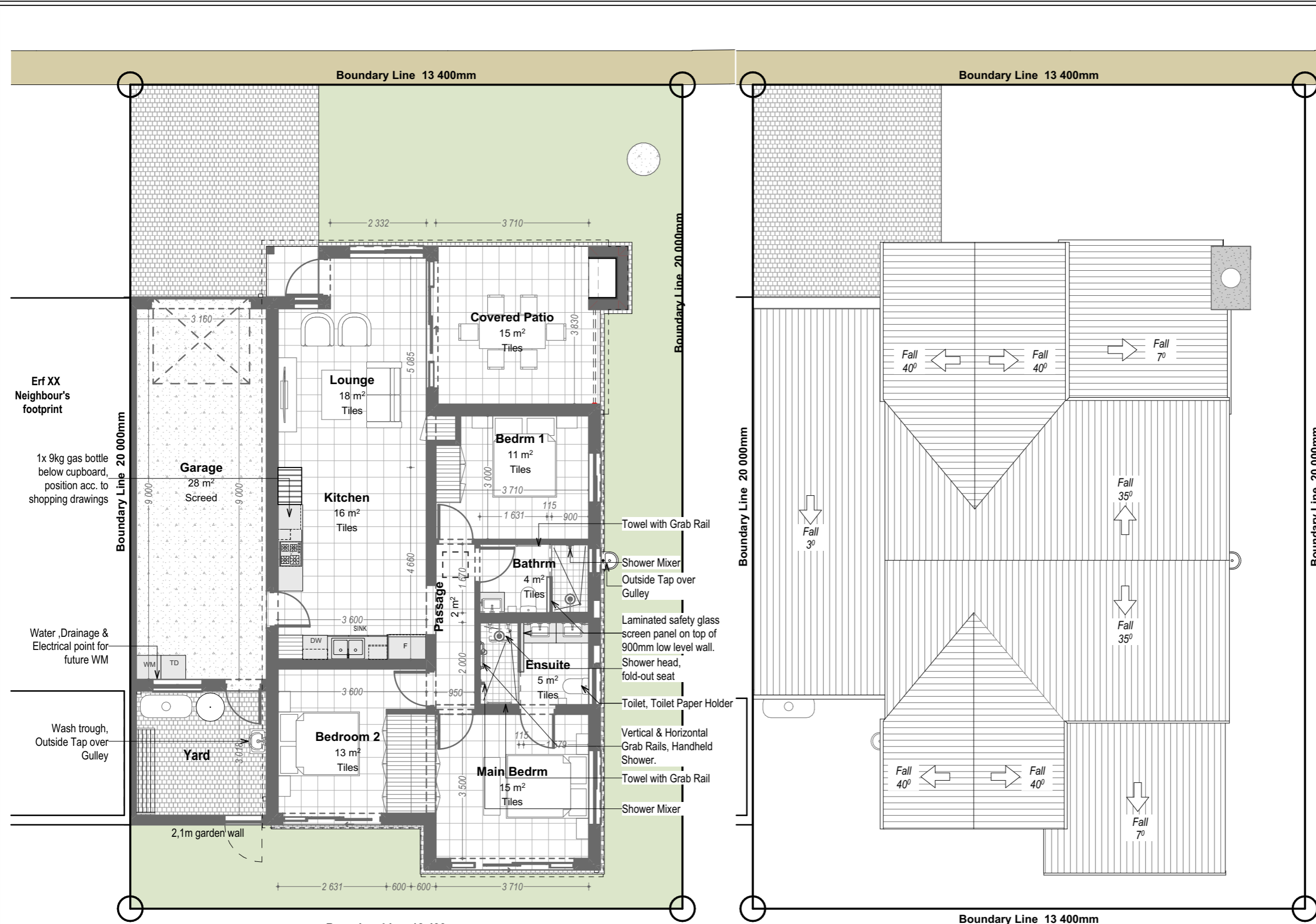
2.1 Ground Floor Plan - (S2) 1:100
