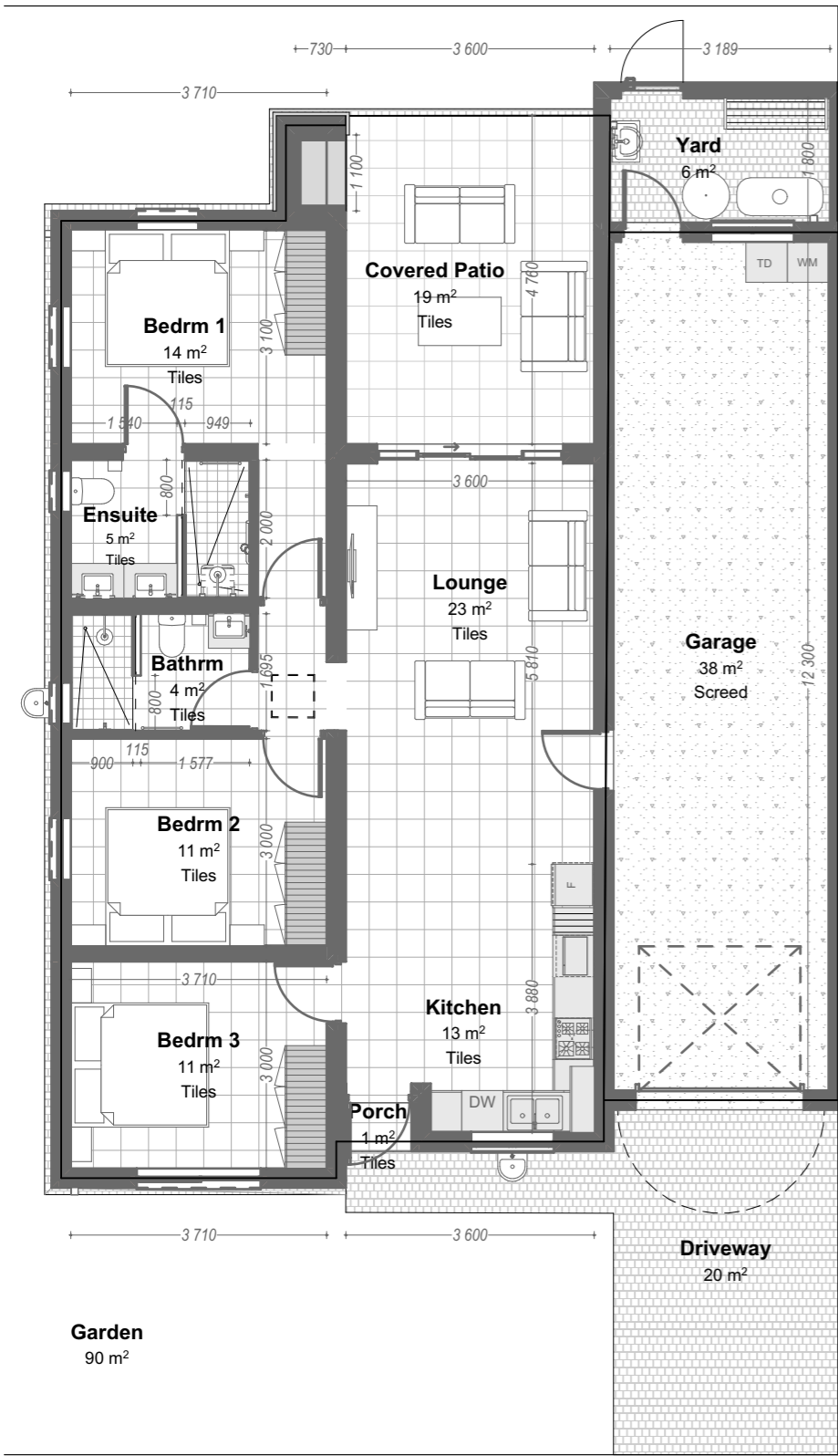
General Floor Plan (G3) 1:100
