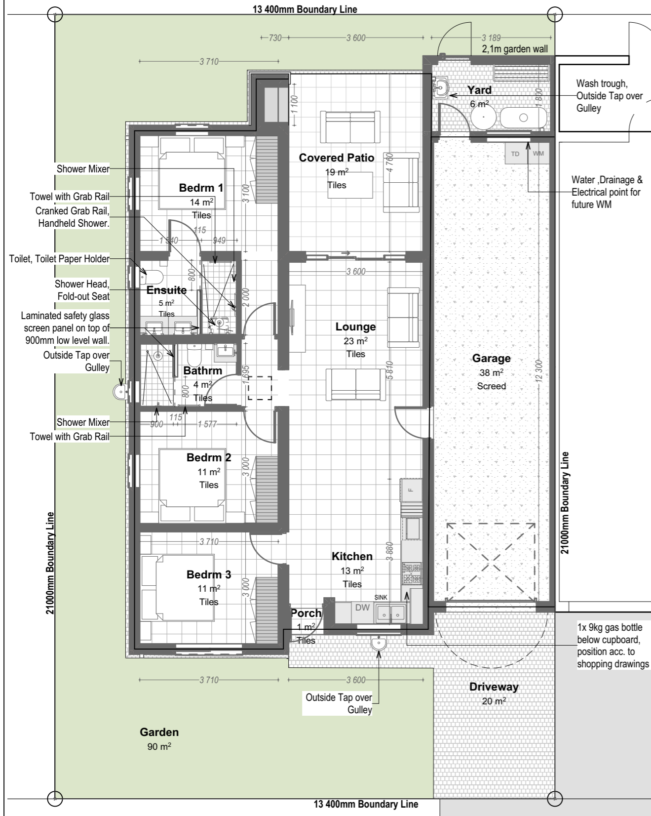
3.1 Ground Floor Plan (G3) 1:100
