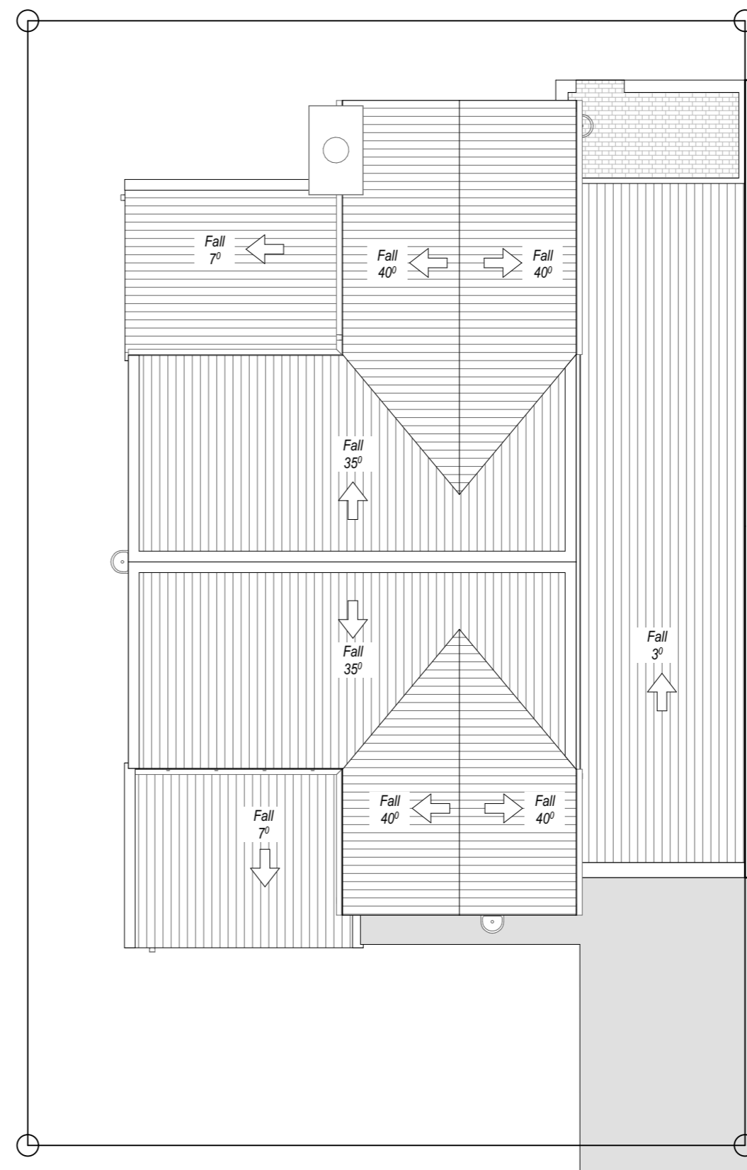
3.1 Roof Plan (G3) 1:100
