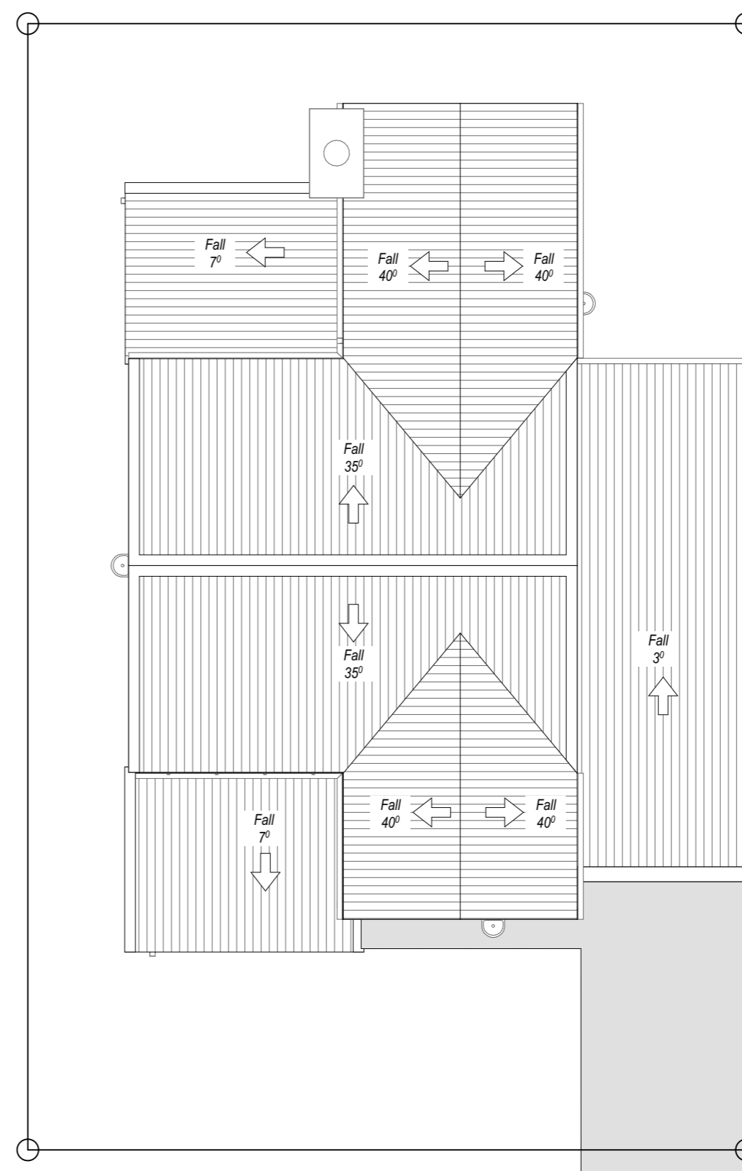
2.1 Roof Plan (G2) 1:100
