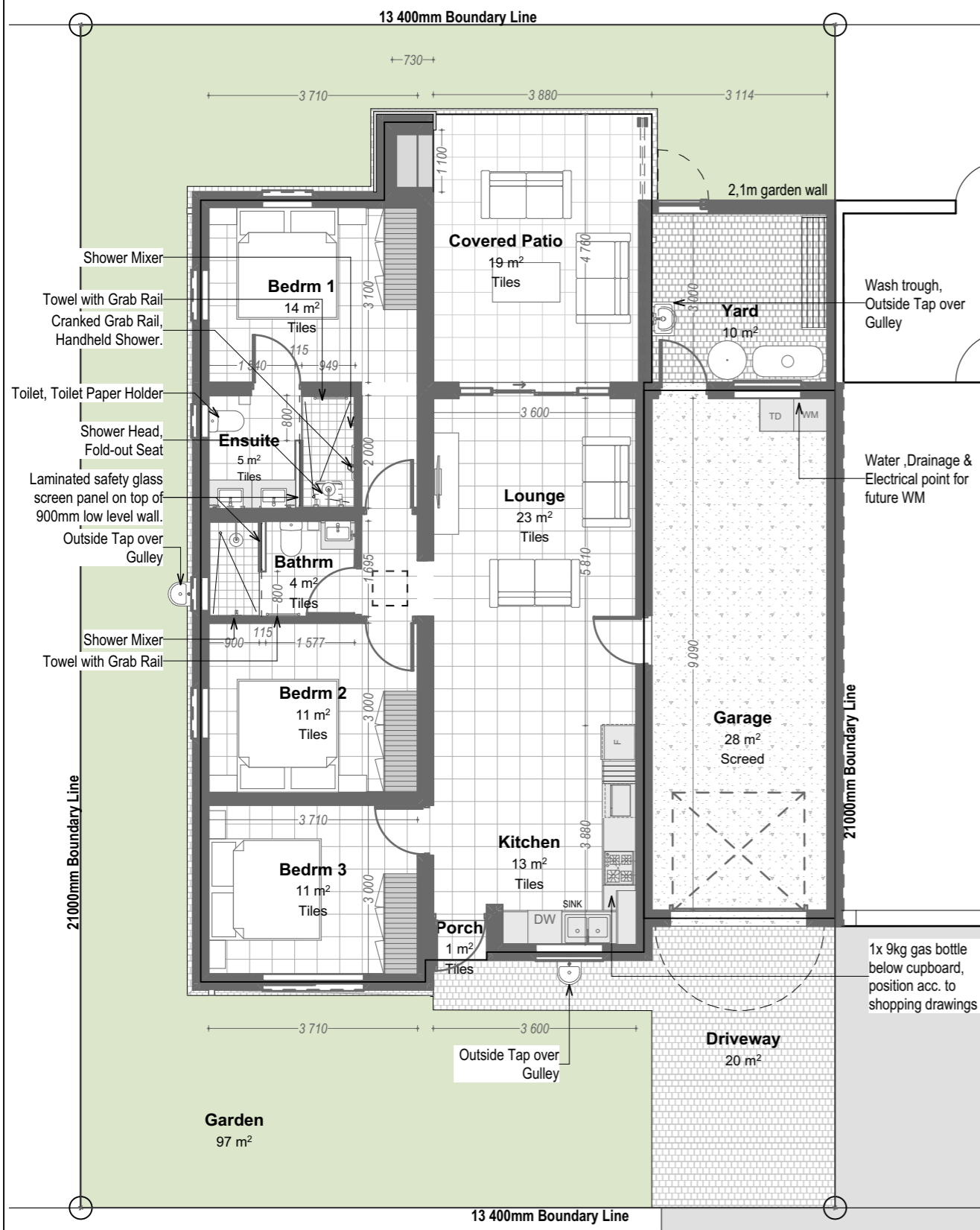
2.1. Ground Floor Plan (G2) 1:100
