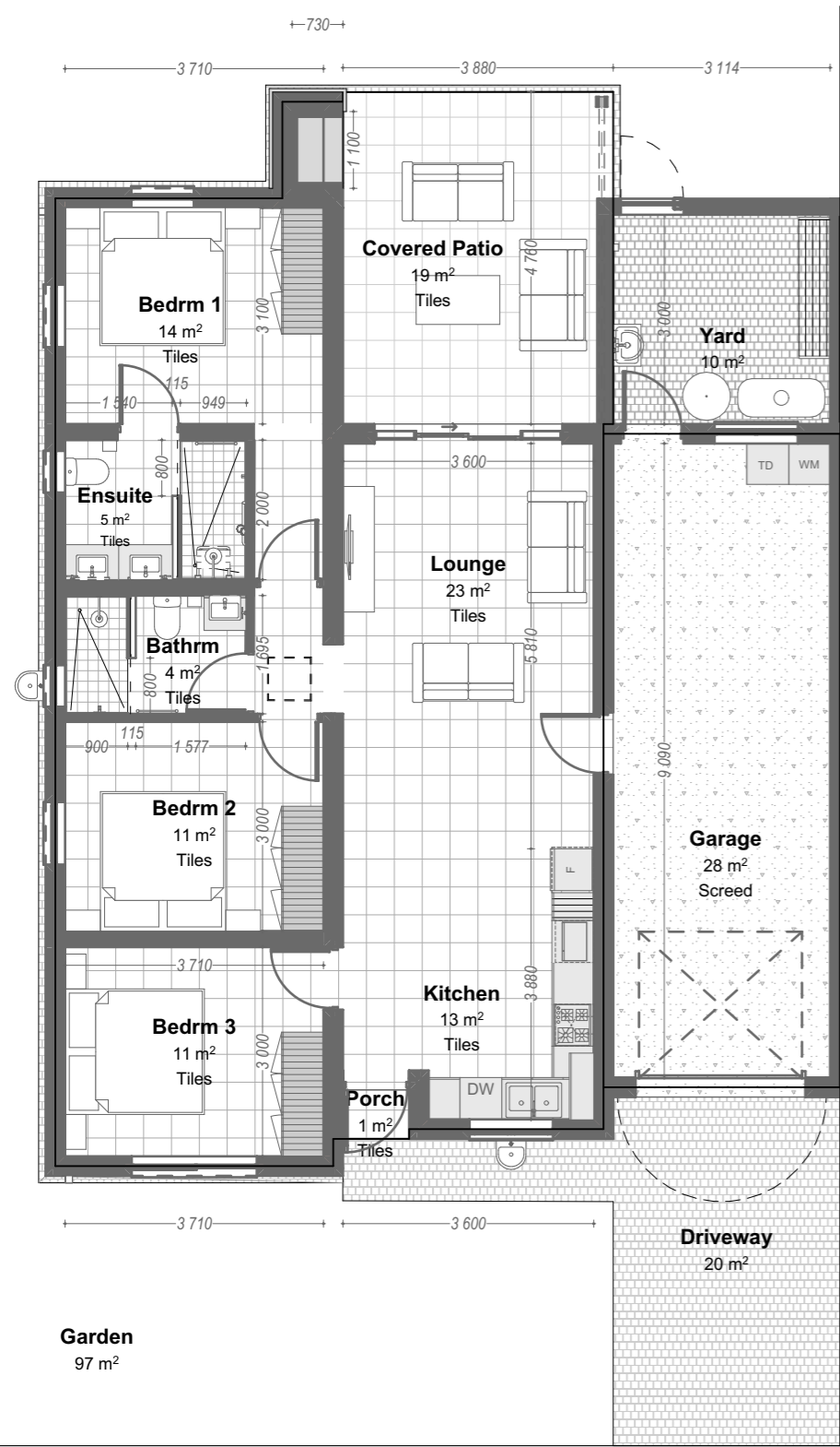
General Floor Plan (G2) 1:100
